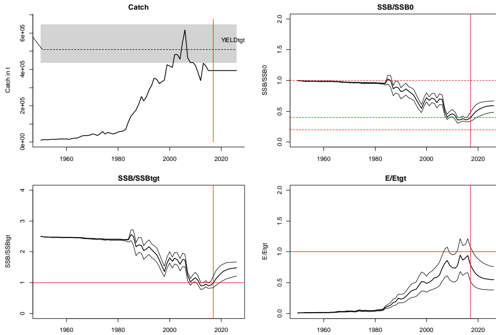
Fig.13. Skipjack tuna: Time series of historical catches (top-left), SSB/SSB0 (top-right), SSB/SSB 40 (bottom-left), and E/E 40B0 (bottom right) estimated from the agreed IO GRID models. In the top-left panel, the shaded area is the estimated 95% CI of the target yield (corresponding to 40%B0). In all other panels, time series include the median and the 95% CI across all models. The vertical line indicates the start of projection period (2017-2026).
